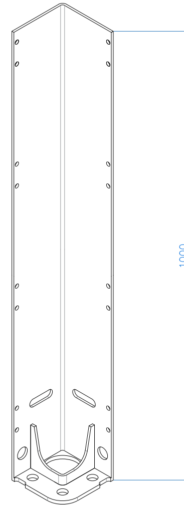
3D INTERNAL BASE PLATE
