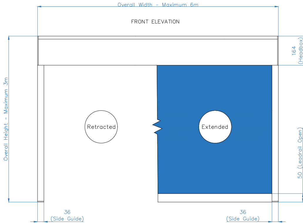
Headbox (for side fix side guide)
