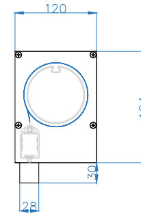
Headbox (for side fix side guide)
